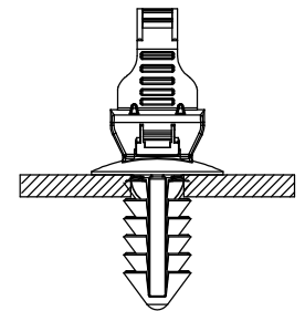
ASSEMBLED VIEW
